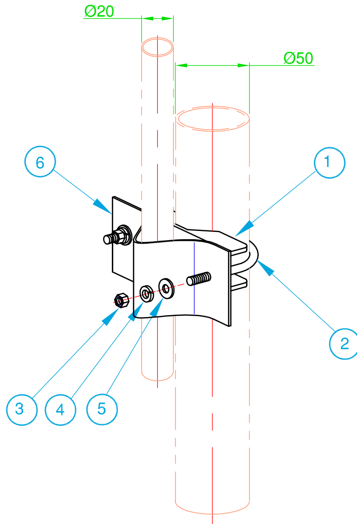
Assembly Sketch UB4SS CLAMP
